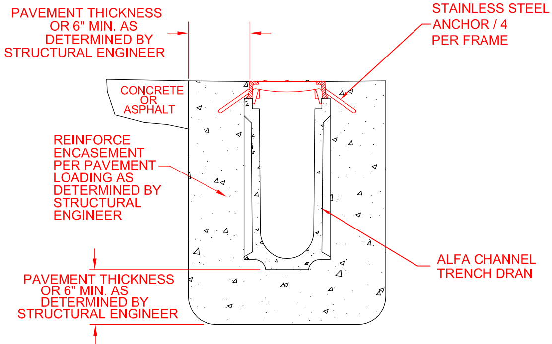
RECOMMENDED ENCASEMENT
