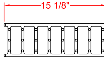
#2542 2-PIECES FRAME & GRATE
