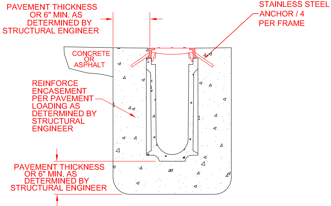
RECOMMENDED ENCASEMENT
