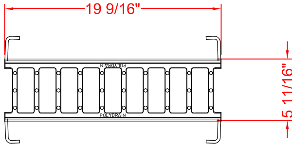
#2552 I-PIECE FRAME & GRATE
