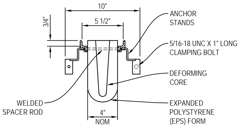
SECTION A-A DO NOT SCALE
